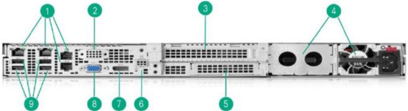
Rear View - Standard for all DL20 Gen11
